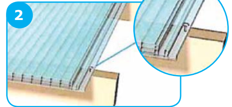
2 Secure the panel onto each batten with a screw.
